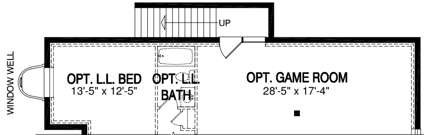
Optional Welled Exit w/ Optional Sunroom
